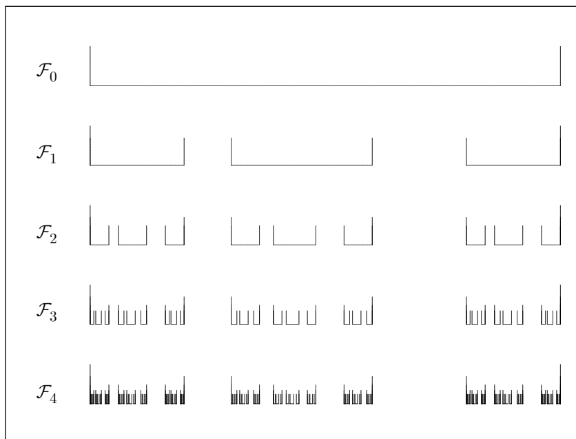
FIGURE 1.1. The first five levels of iteration of the generalized Cantor set with parameters \rho_1 = 0.2, b_1 = 0, \rho_2 = 0.3, b_2 = 0.3, \rho_3 = 0.2, b_3 = 0.8 . \alpha for this example is approximately 0.7524. Note that vertical bars have been added at island-lake boundaries.
