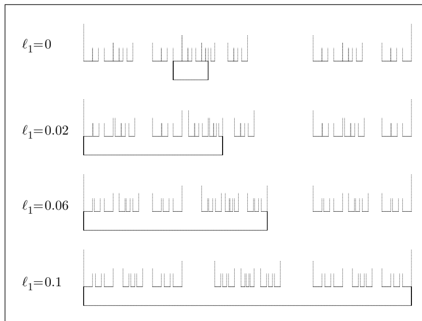
FIGURE 2.2. The island configurations which give rise to the maximum densities for the i.f.s. of Figure 2.1 for four representative values of \ell_1 .
